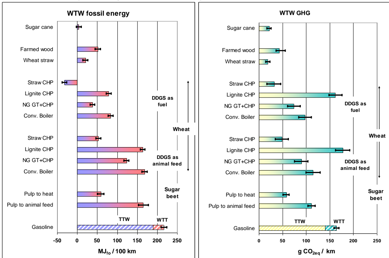
Figure 5.1.5-1 WTW fossil energy requirement and GHG emissions for ethanol pathways (2010+ vehicles)
