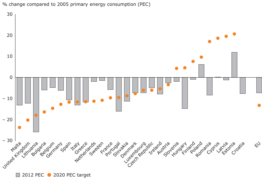
Figure 6.4 2012 primary energy consumption and 2020 national targets compared to 2005 levels
