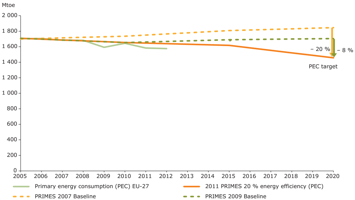
Figure 6.2 Primary energy consumption baseline in the EU-27 (PRIMES 2007, PRIMES 2009) in comparison with the 2020 energy efficiency target
