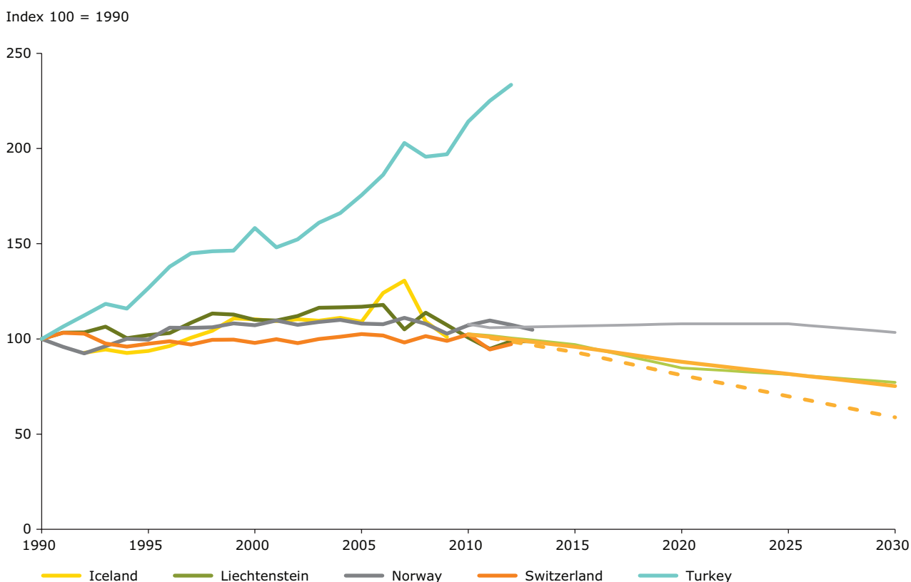
Figure 4.12 GHG emission trends and projections in other EEA member countries, 1990–2030
