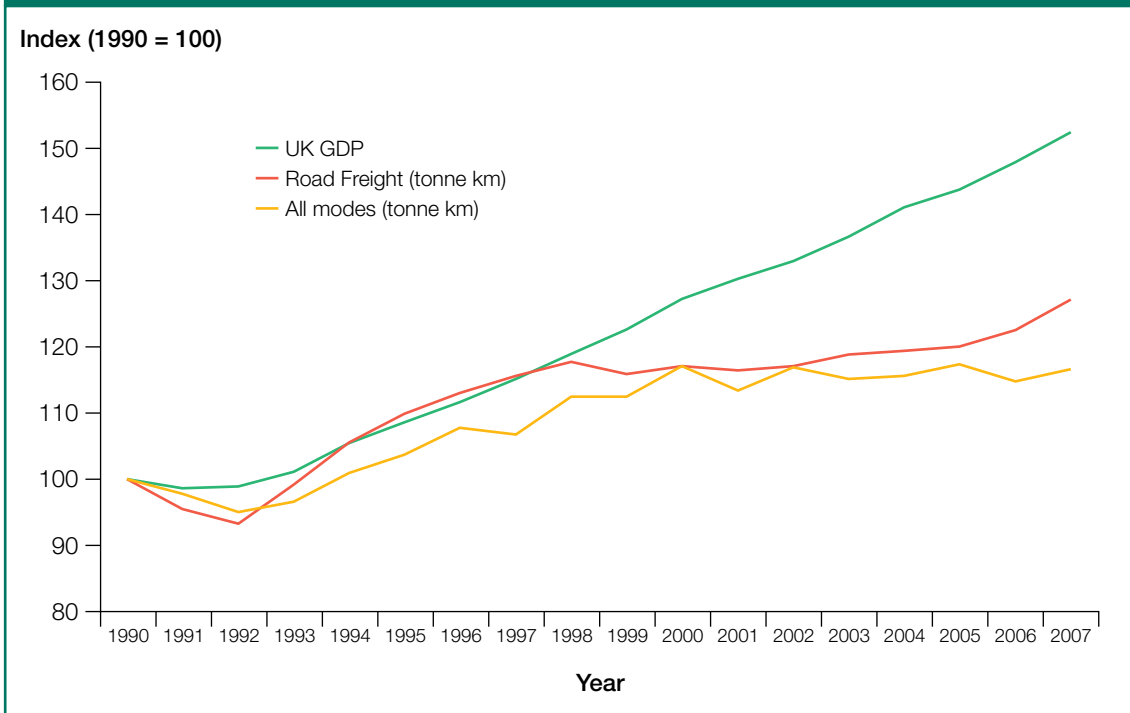
Figure 1 UK GDP and tonne kilometres, 1990–2007
