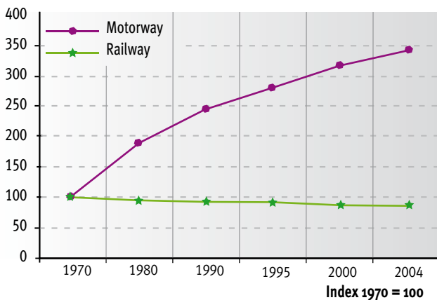
Length of rail lines and motorways (km) in EU-15 (1970 = 100)
