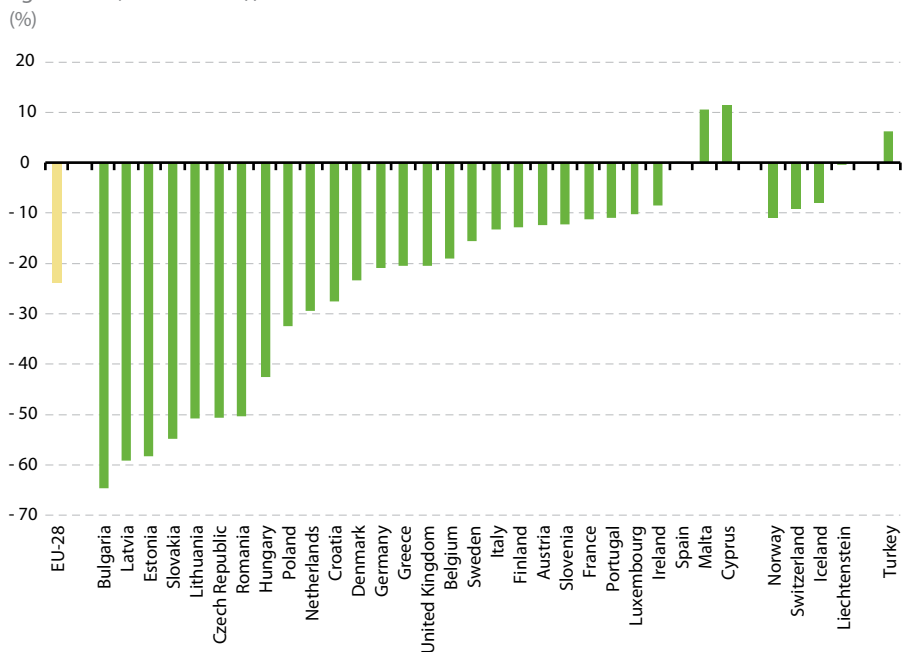
Figure 5.18: Change in aggregated emissions of methane and nitrous oxide from agriculture, 1990–2012 (†)
