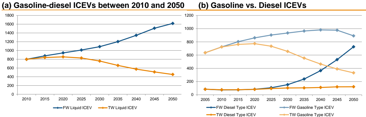
Figure 33 Technology mix for LDV gasoline-diesel ICEVs (million)
