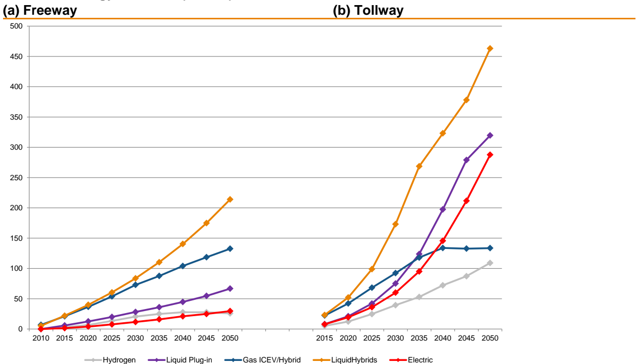
Figure 34 Other technology LDV cars (million)
