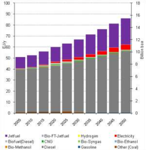
Figure 23 Fuel in other surface transport and aviation (a) Demand between 2010 and 2050
