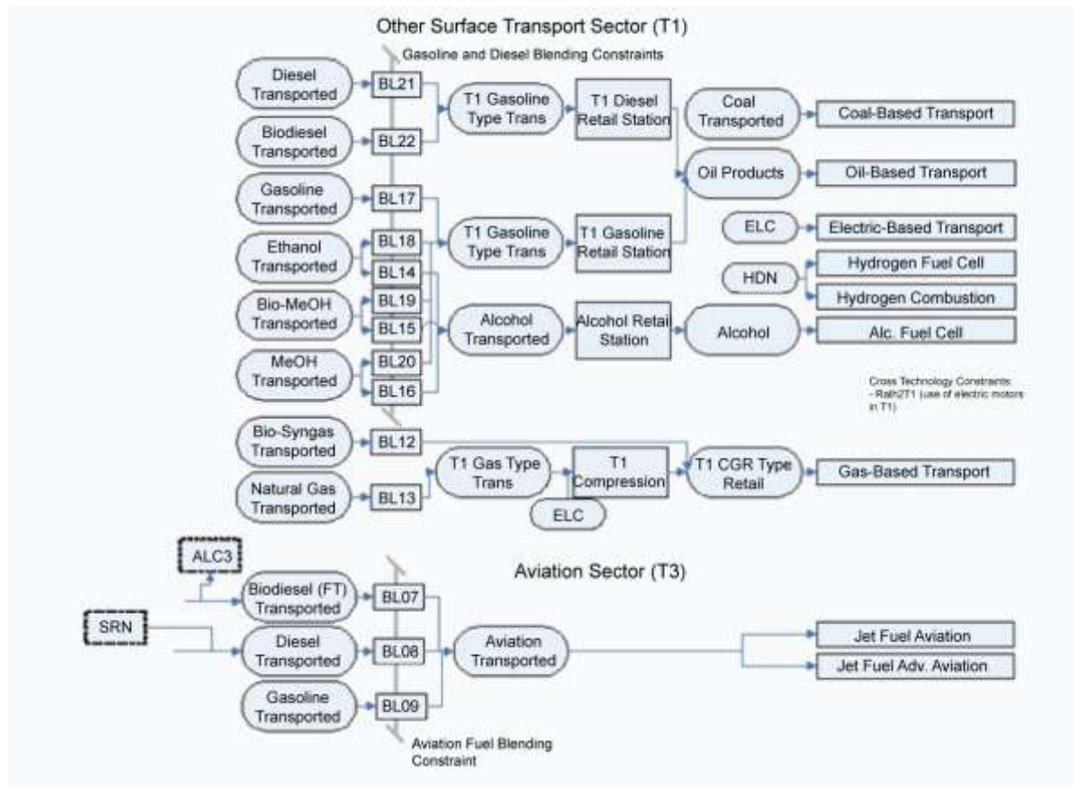
Figure 15 Other surface transport and aviation sectors in GMM
