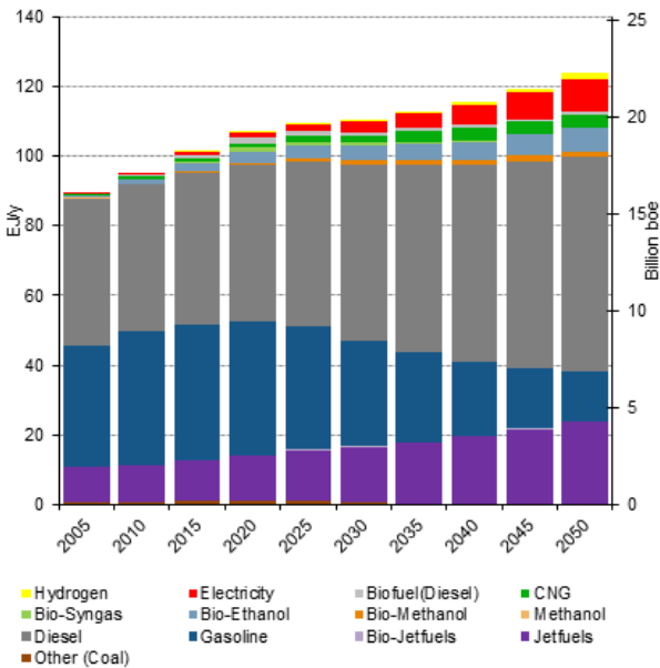
Figure 24 Fuels in all transport (a) Demand between 2010 and 2050
