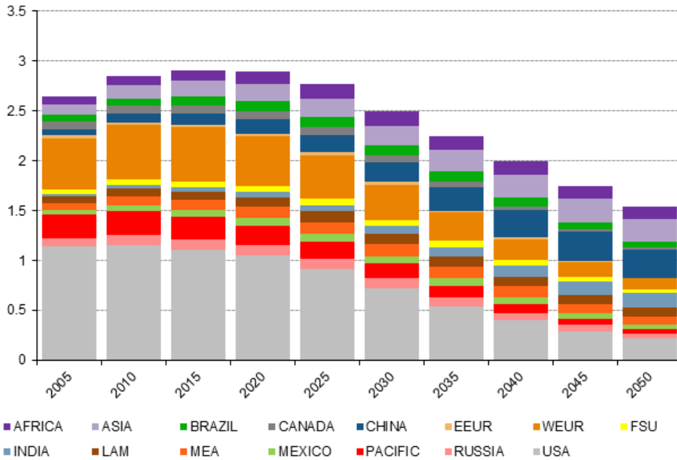
Figure 26 CO 2 emissions from cars (GtCO 2 /y)
