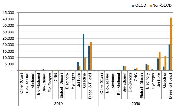
(b) Demand of OECD vs. non-OECD (EJ)
