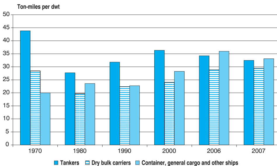
Figure 15 Ton-miles per deadweight ton (dwt) of the world fleet, by vessel types, selected years
