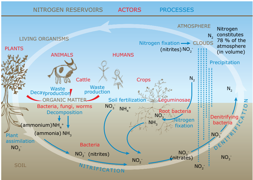
Figure 10.1 The nitrogen cycle
