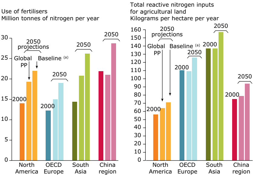
Figure 10.2 Use of fertilisers and total reactive nitrogen inputs on agricultural land
