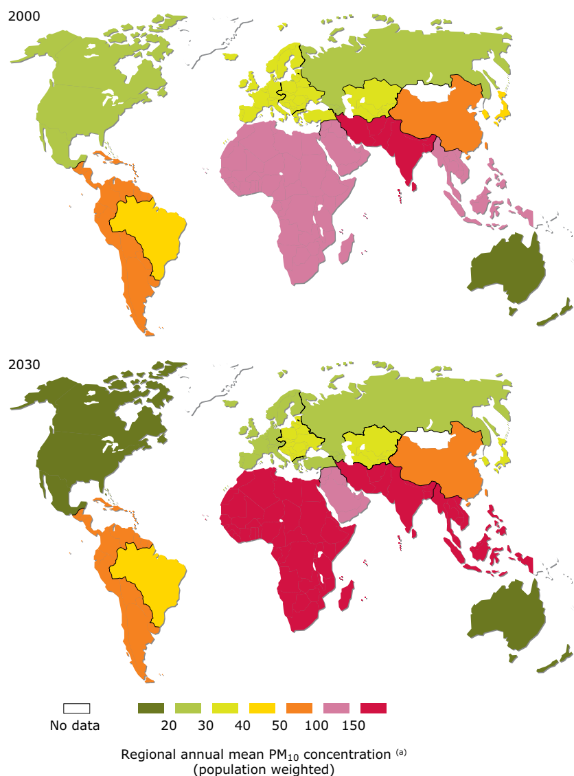
Map 10.1 Particulate matter pollution
