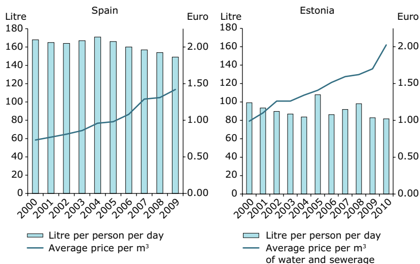
Figure 8.3 Water pricing and household water use between 2000 and 2009/2010 in Spain (left) and Estonia (right)
