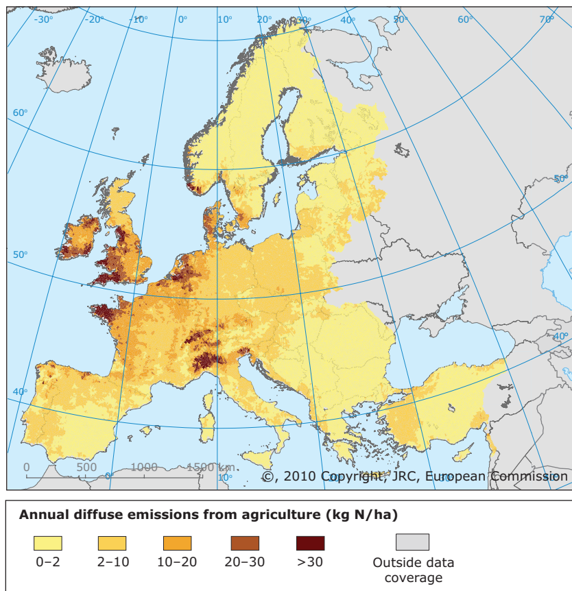
Map 4.2 Annual diffuse emissions of nitrogen to freshwater from agriculture
