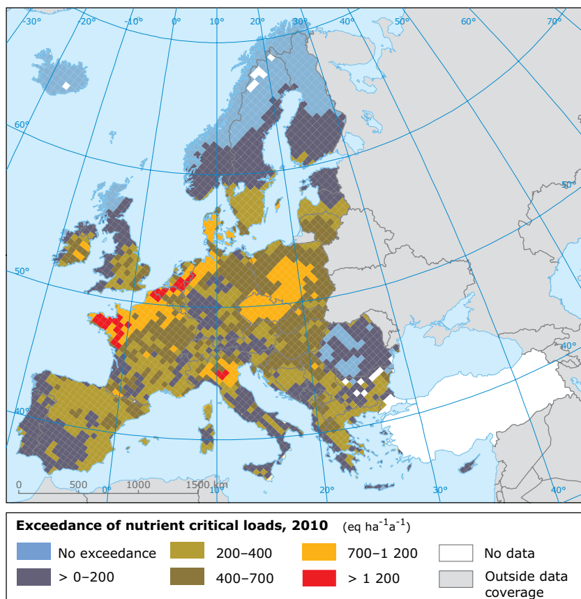
Map 4.1 Exceedance of the critical nitrogen loads for eutrophication in Europe, 2010
