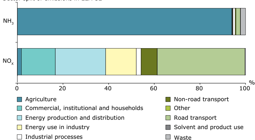
Figure 4.4 Sectoral contributions of air emissions of acidifying pollutants in EEA member countries
